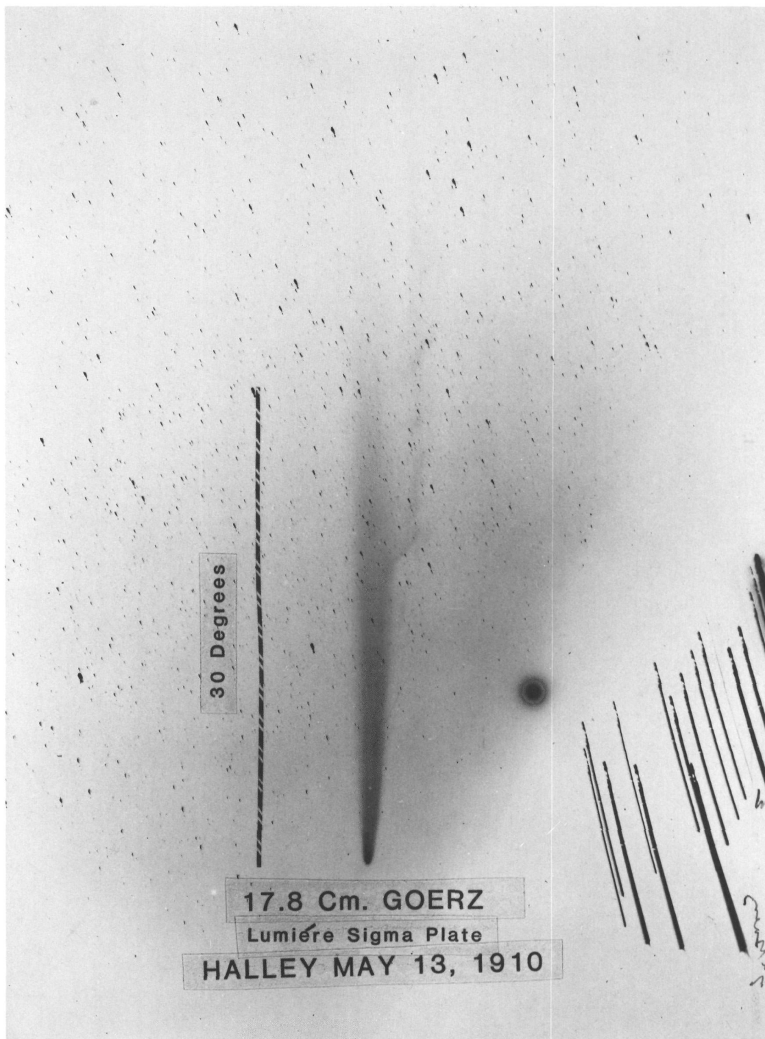
Figure 4. Photograph of Comet Halley obtained on May 13, 1910.
